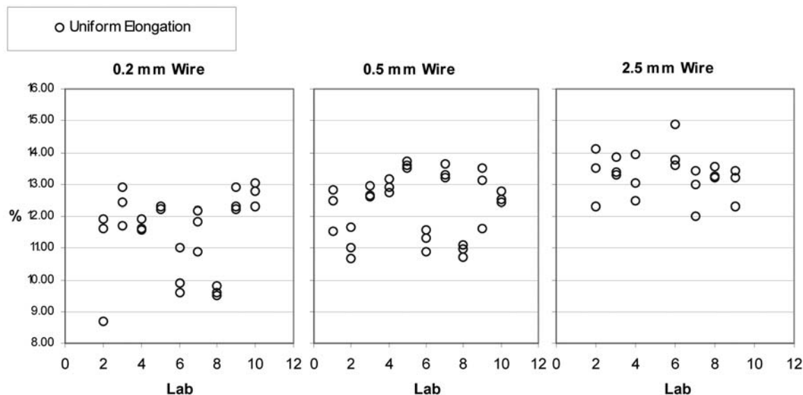
FIG. X2.5 Uniform Elongation
