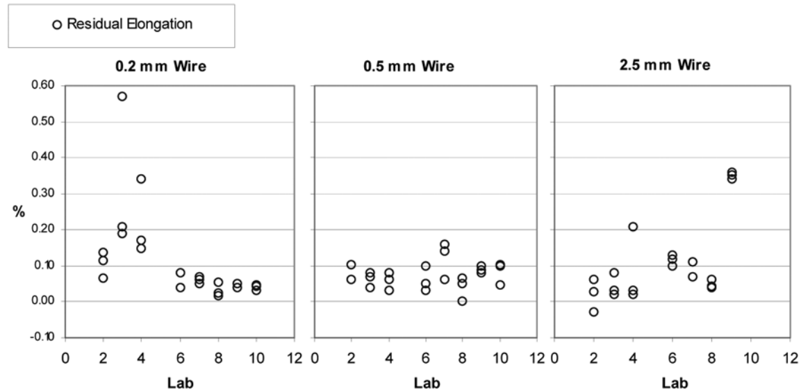
FIG. X2.3 Residual Elongation
